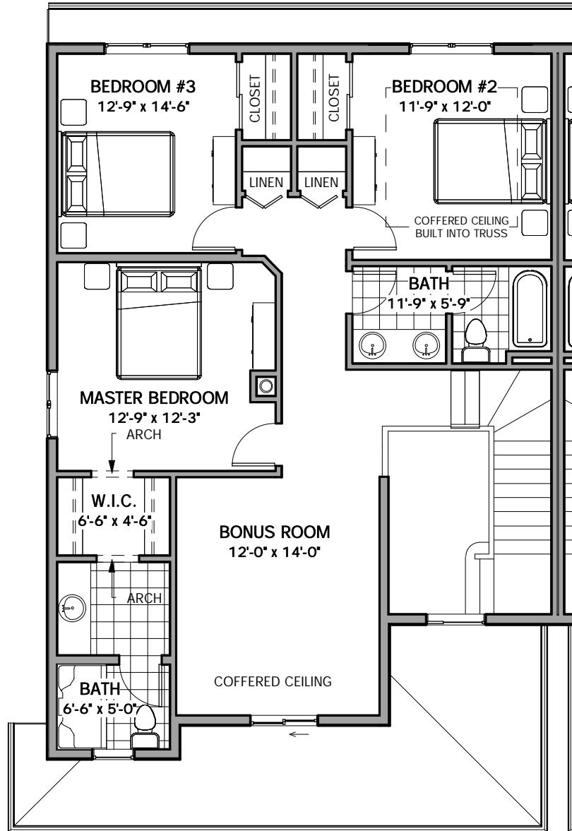
Lot 9 - Second Floor 1/8" = 1'-0"
